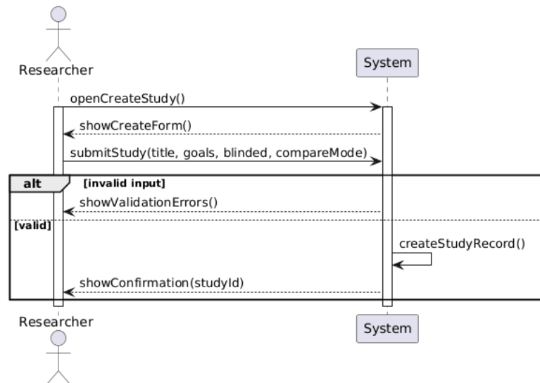
Create Study — System Sequence Diagram
